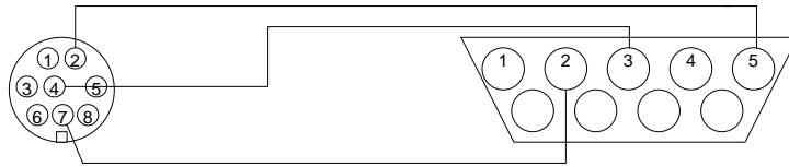
db9 Male To GPS
