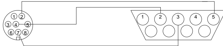
db9 Female To Computer
