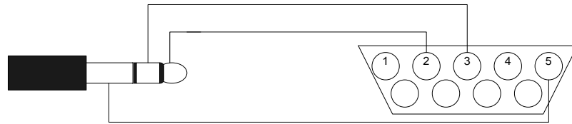
db9 Male To GPS
